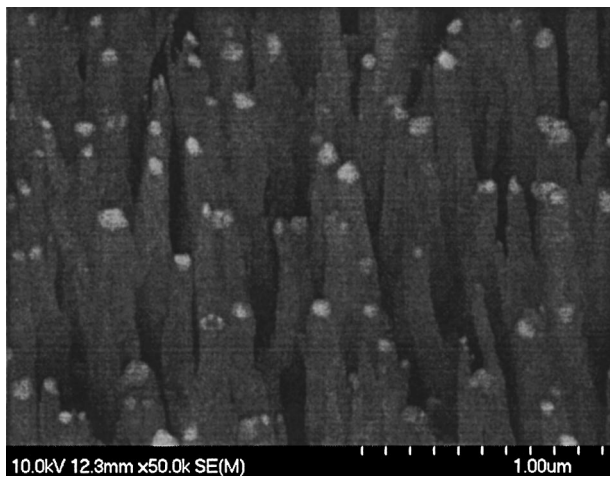
FIG. 1. Scanning electron microscopy (SEM) images of a typical VACNF forest grown from a Ni/Fe catalyst stripe.
