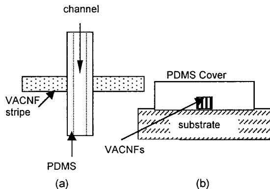
FIG. 2. (a) A top view schematic of the PDMS channel and VACNF membrane. PDMS channels were placed over the nanofiber stripes. (b) A cross-sectional view along the axis of fluid flow.
