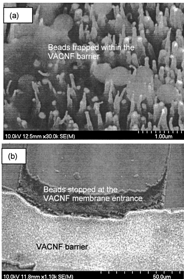
FIG. 4. Postexperiment SEM images of (a) 500 nm beads trapped within the nanofiber array and (b) 750 nm beads stopped by the nanofiber array.
