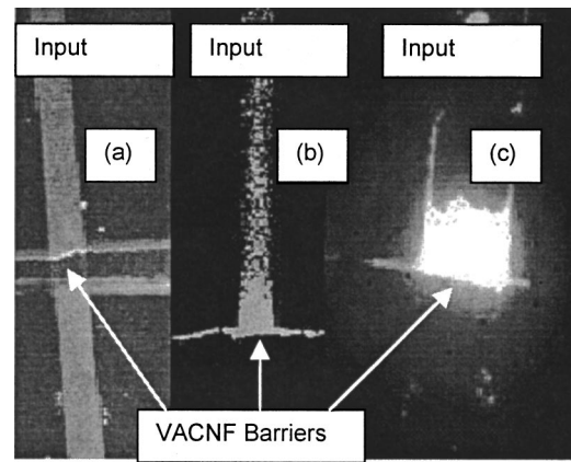
FIG. 3. Fluorescence microscope images of (a) 100 nm beads flowing in a 100 \mu m wide channel; (b) 500 nm beads flowing in a 100 \mu m wide channel; and (c) 750 nm beads flowing in a 50 \mu m wide channel.
